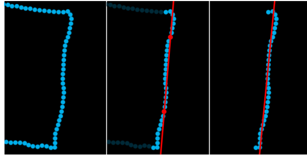
Figure 4. From left to right: Original contour points, line result after Ransac fitting, revised line result after Least Squares fitting on Ransac supporters
