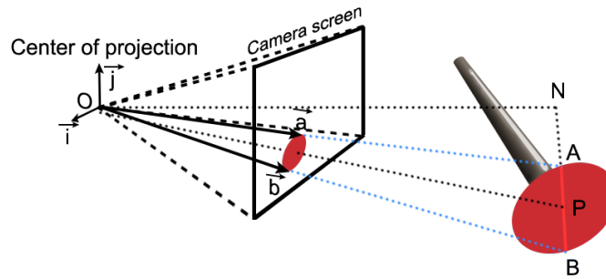
Figure 7. Pencil marker detection process
