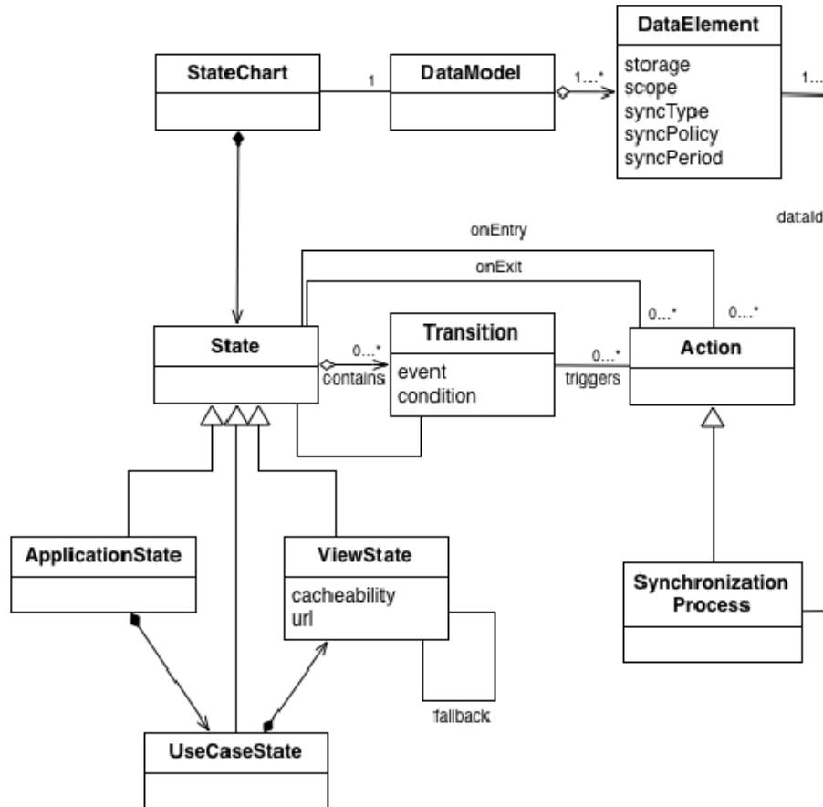
Figure 1- Class diagram for the navigation model
