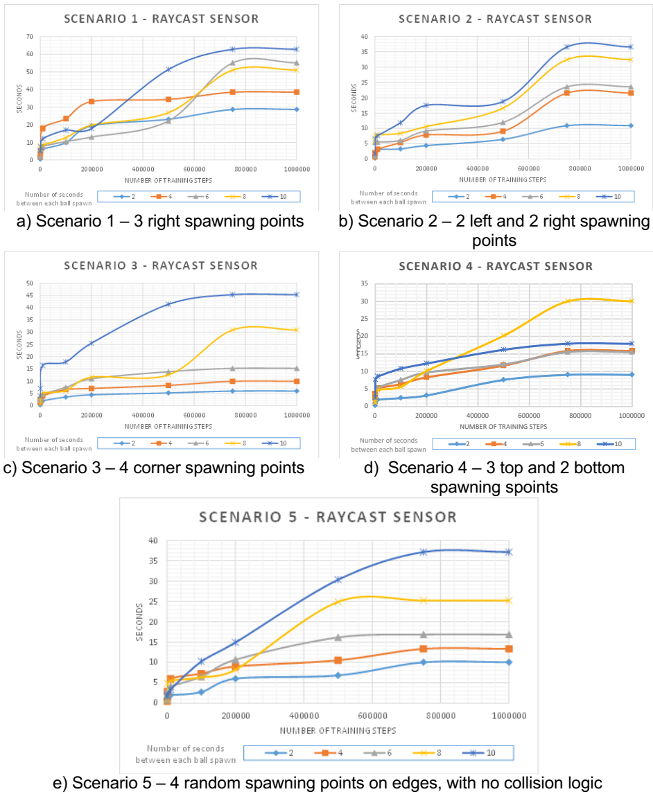
Figure 5. Charts showing the runtimes in seconds for scenarios from 1 to 5, using Raycast sensor, with varying numbers of seconds between ball spawn (2 to 10)
